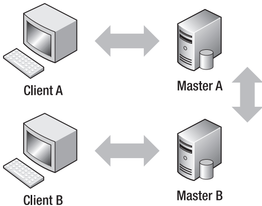
Figure 11–4. Master/master replication
